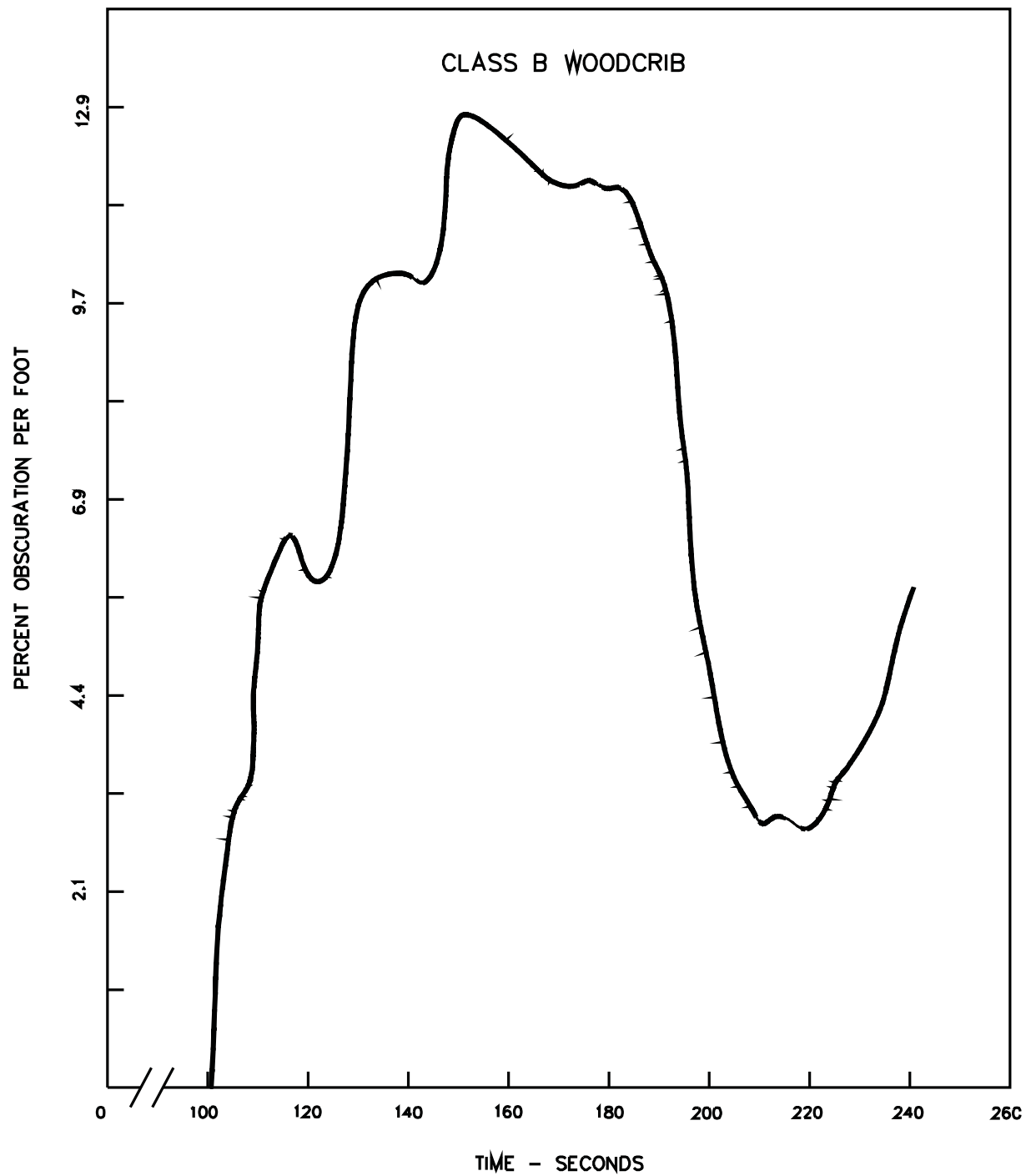
Figure 44.7 Woodcrib profile
