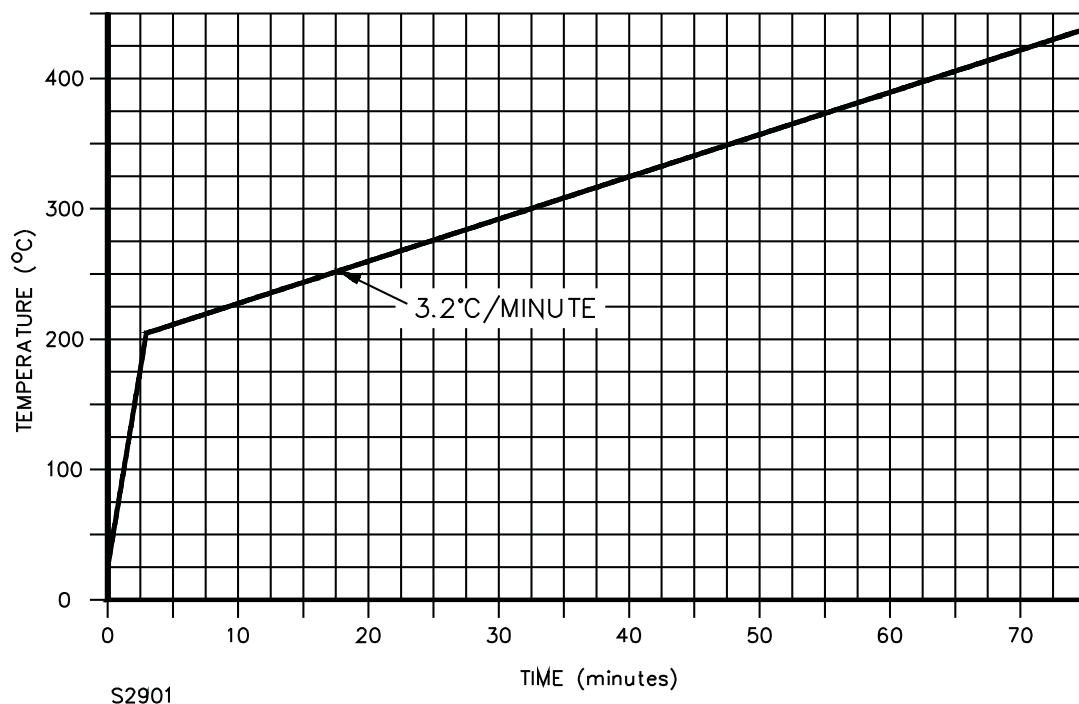
Figure 45.1 Hotplate temperature profile
