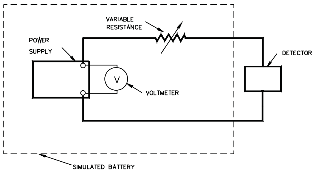
Figure 35.1 Test circuit
