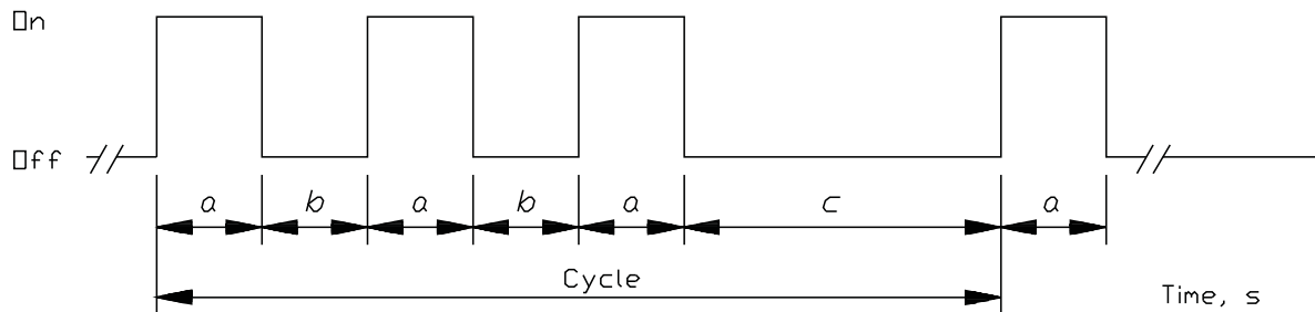
Figure 34.1 Standardized alarm signal temporal pattern
