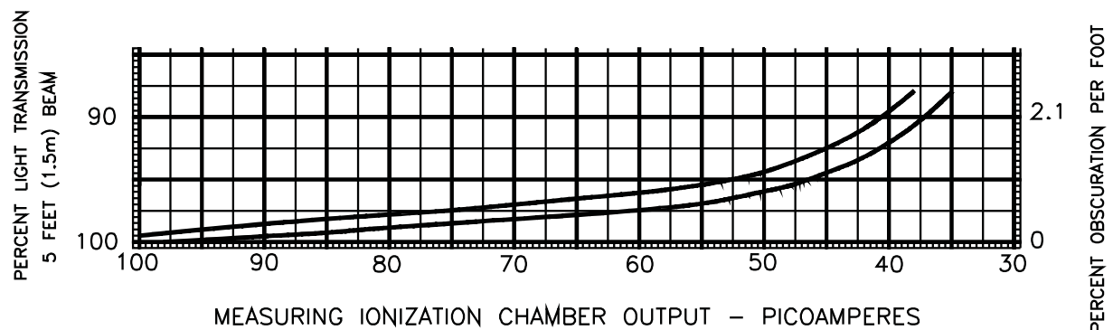
Figure 38.1 Smoke entry test limits – aerosol – 150 fpm
