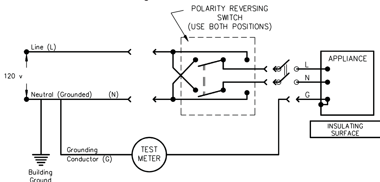
Figure 52.1 Leakage current measurement circuit
