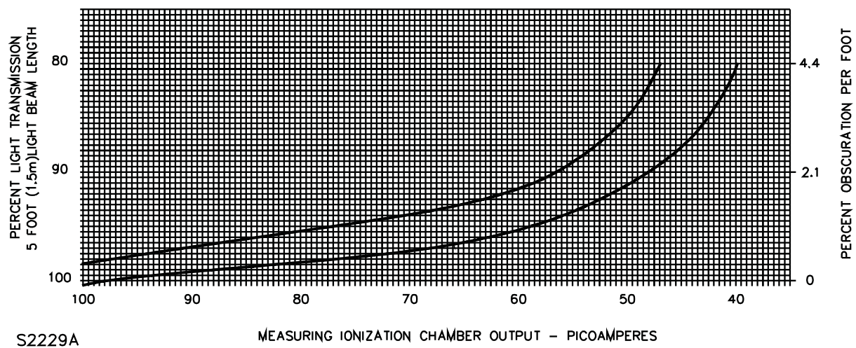
Figure 50.2 Sensitivity test limits – 49°C ambient– aerosol – 32 fpm
