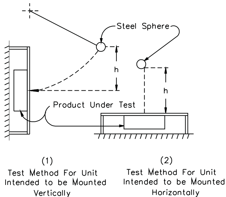
Figure 60.1 Jarring test
