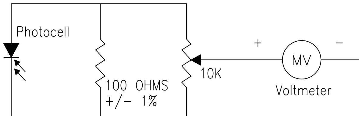
Figure 37.3 Potentiometer placement
