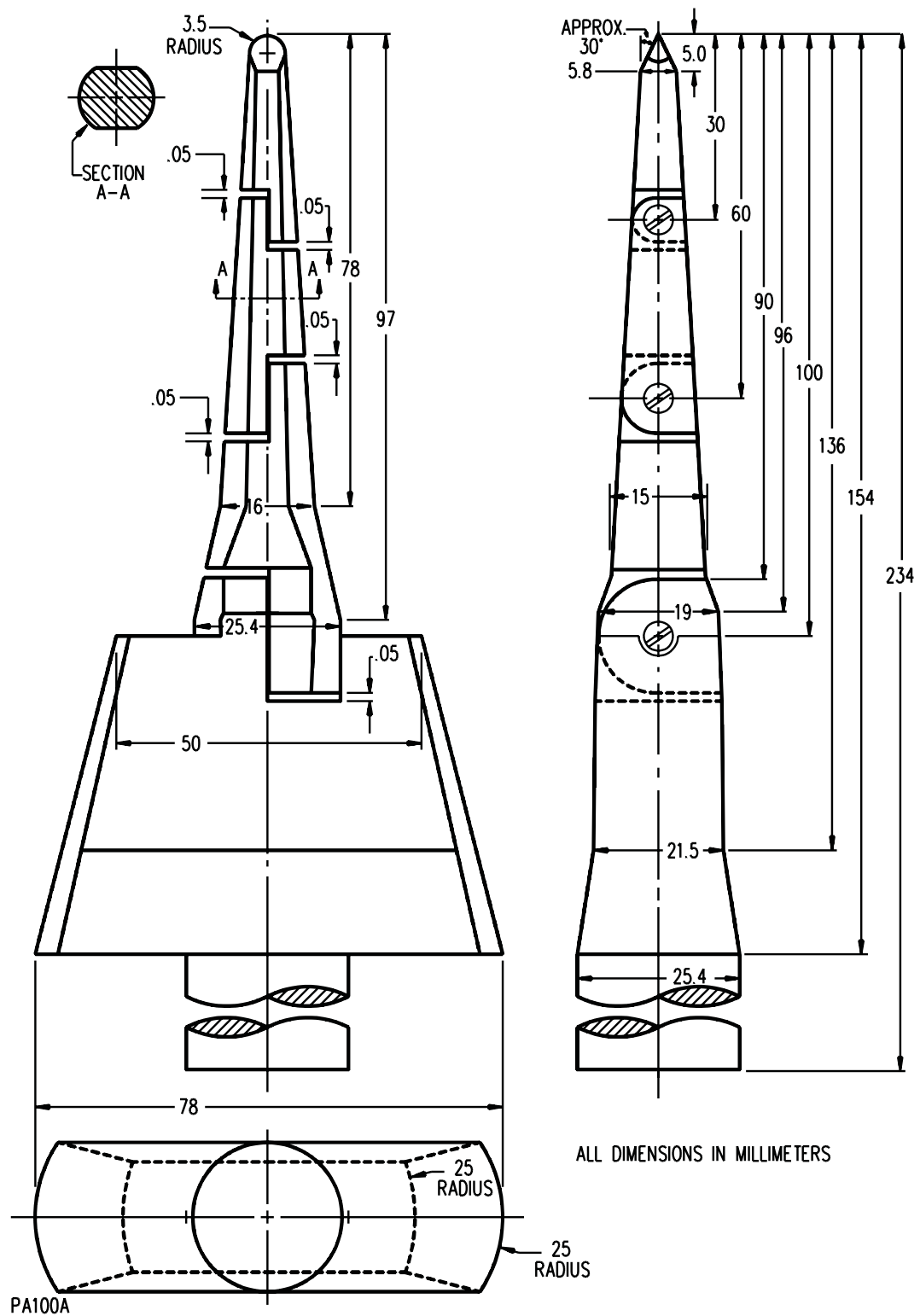
Figure 70.1 Articulated probe
